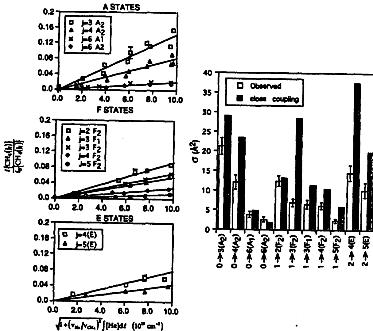
Fig. 3. Sample data for He + CH 4 scattering at E com = 460 cm -1
